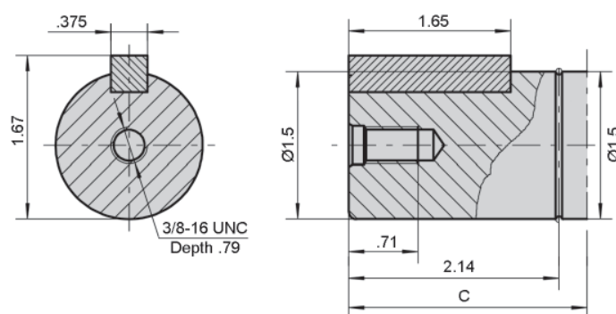
G32 - 1 1/2" Keyed
