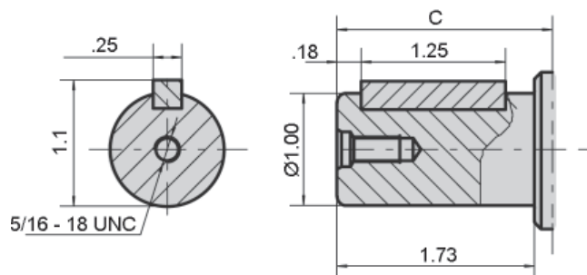
RW - 1" Keyed
